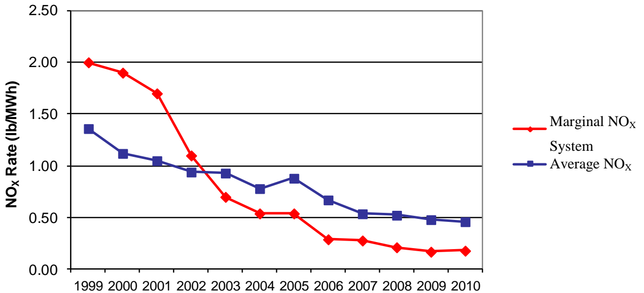
Figure 5.5: 1999 – 2010 Calculated New England Annual Average System NO x Emission Rate vs. Marginal NO x Emission Rate (lb/MWh)
