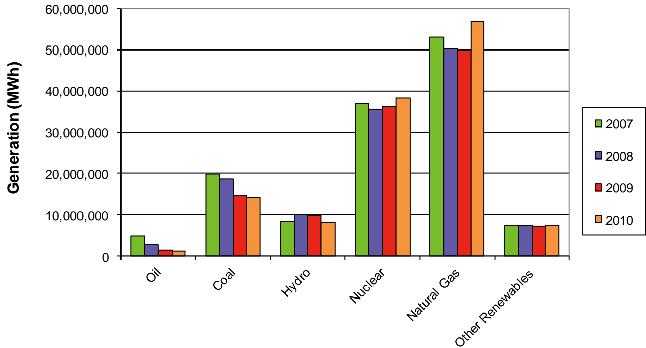
Figure 4.2 : 2007-2010 Generation by Selected Fuel Types
