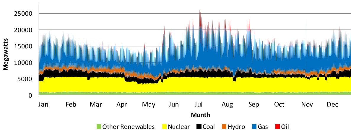
Figure 3.1: New England 2010 Hourly Generation
