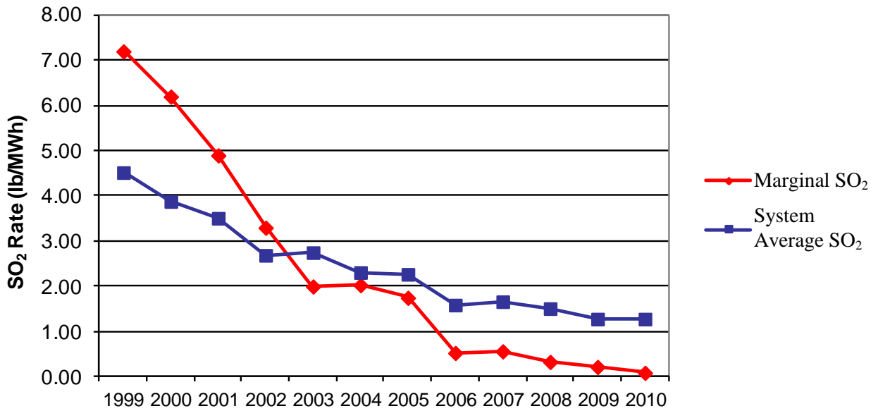
Figure 5.6: 1999 – 2010 Calculated New England Annual Average System SO 2 Emission Rate vs. Marginal SO 2 Emission Rate (lb/MWh)
