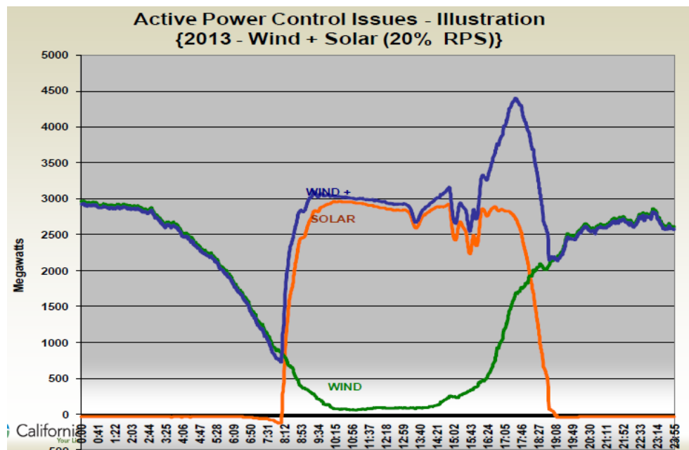
Exhibit 1-3: Combined wind and solar production profiles in California under a 20% RPS
