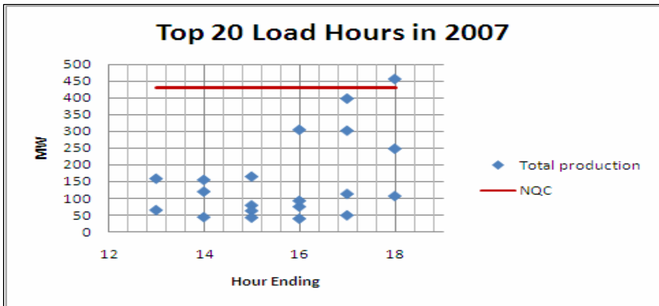
Exhibit 2-8: VER Peak Load Production in CAISO, 2007
