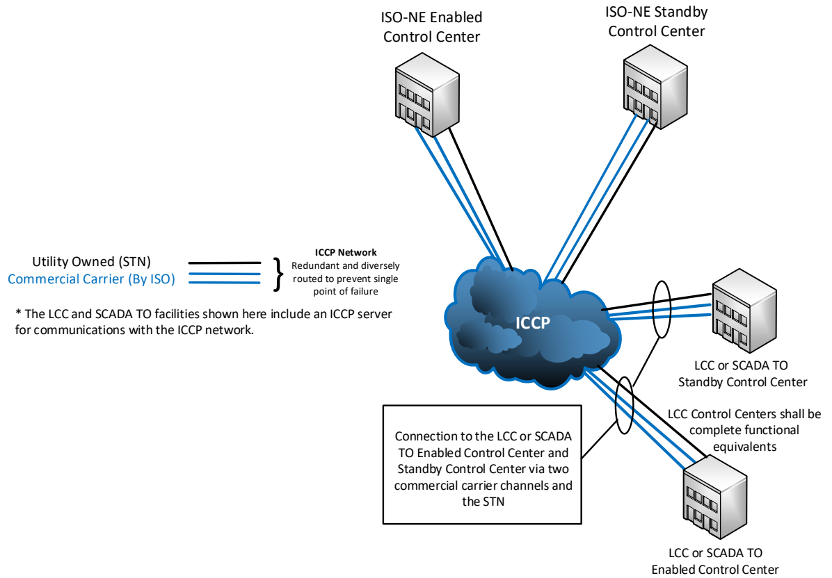
Diagram 1 – New England ICCP Network
