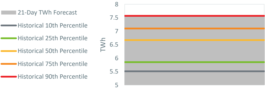
Total 21 Day Energy Demand
