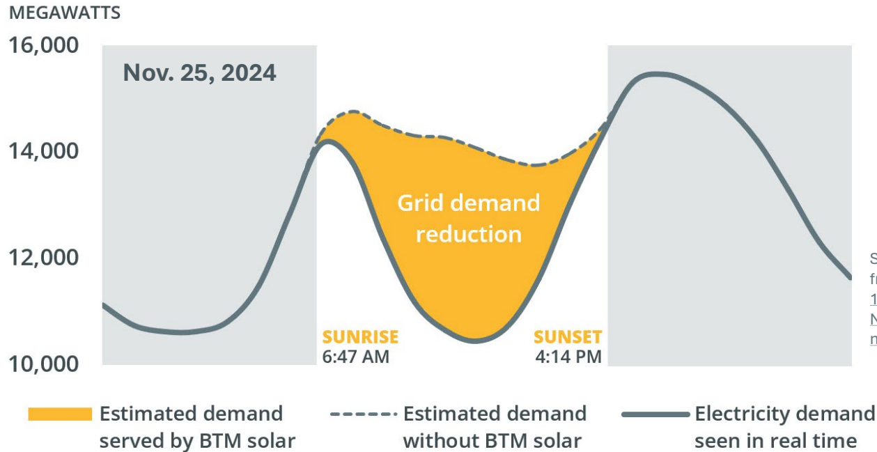
Grid demand reduction from behind-the-meter (BTM) solar
