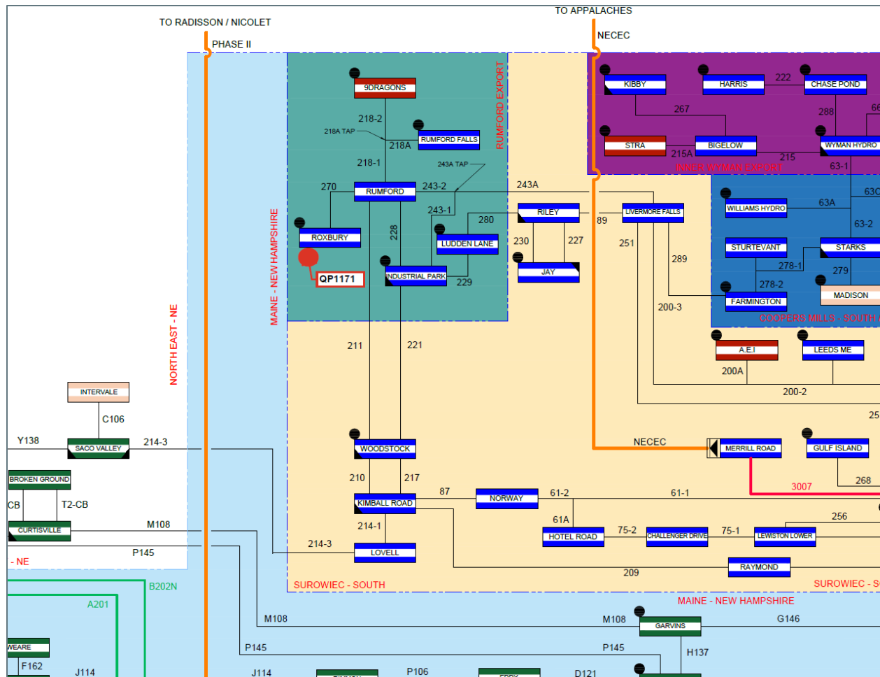
Figure 1-5: QP1171 System Diagram One-Line
