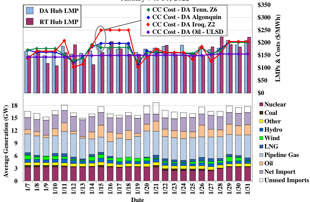
Figure 12: Generation by Fuel Type and Imports to New England January 7 to 31, 2022
