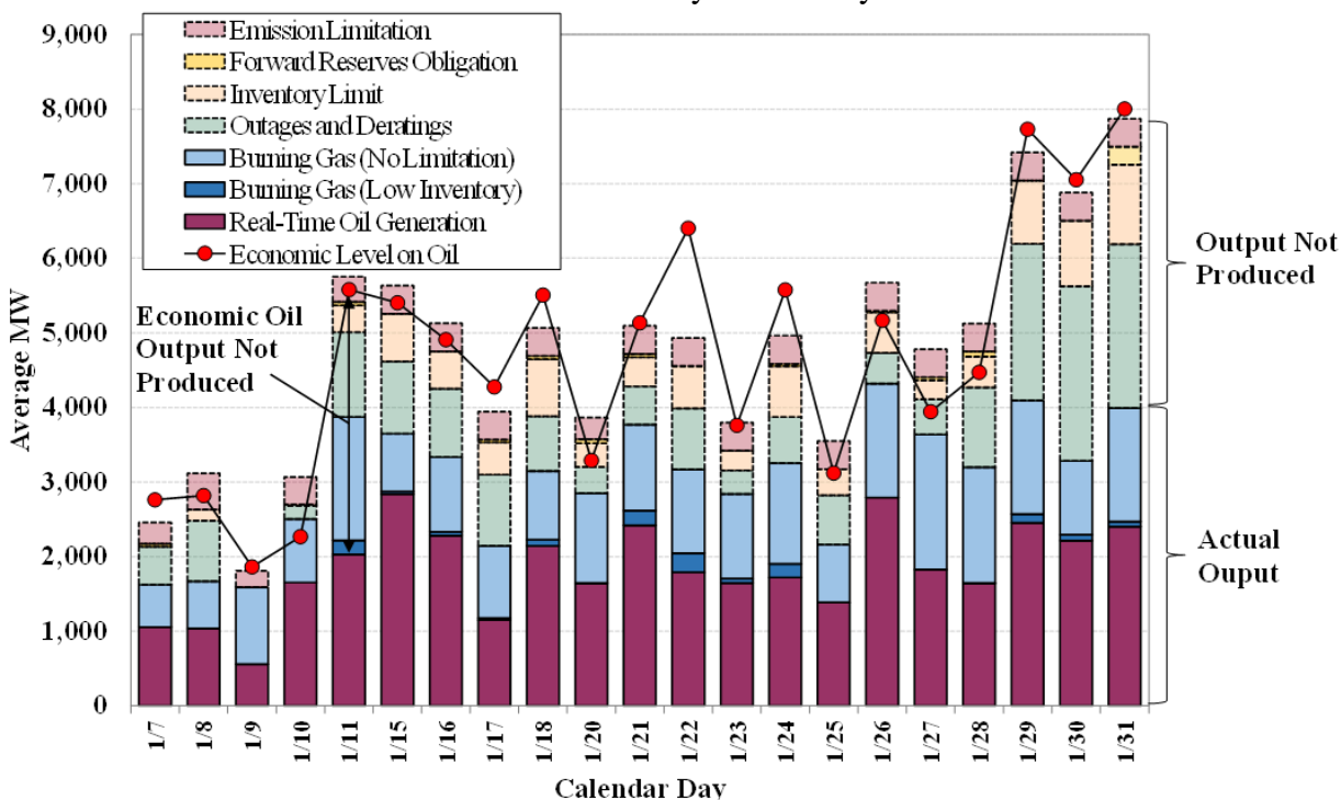
Figure 13: Utilization of Oil-Fired and Dual-Fuel Capacity Selected Calendar Days in January 2022
